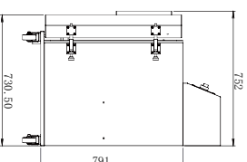
DZL-600 Vertical Chamber Vacuum Packing Machine 立式真空包装机
